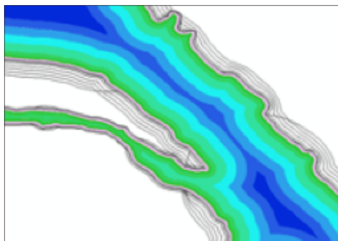
Figure 3-2: Apply Buffers
